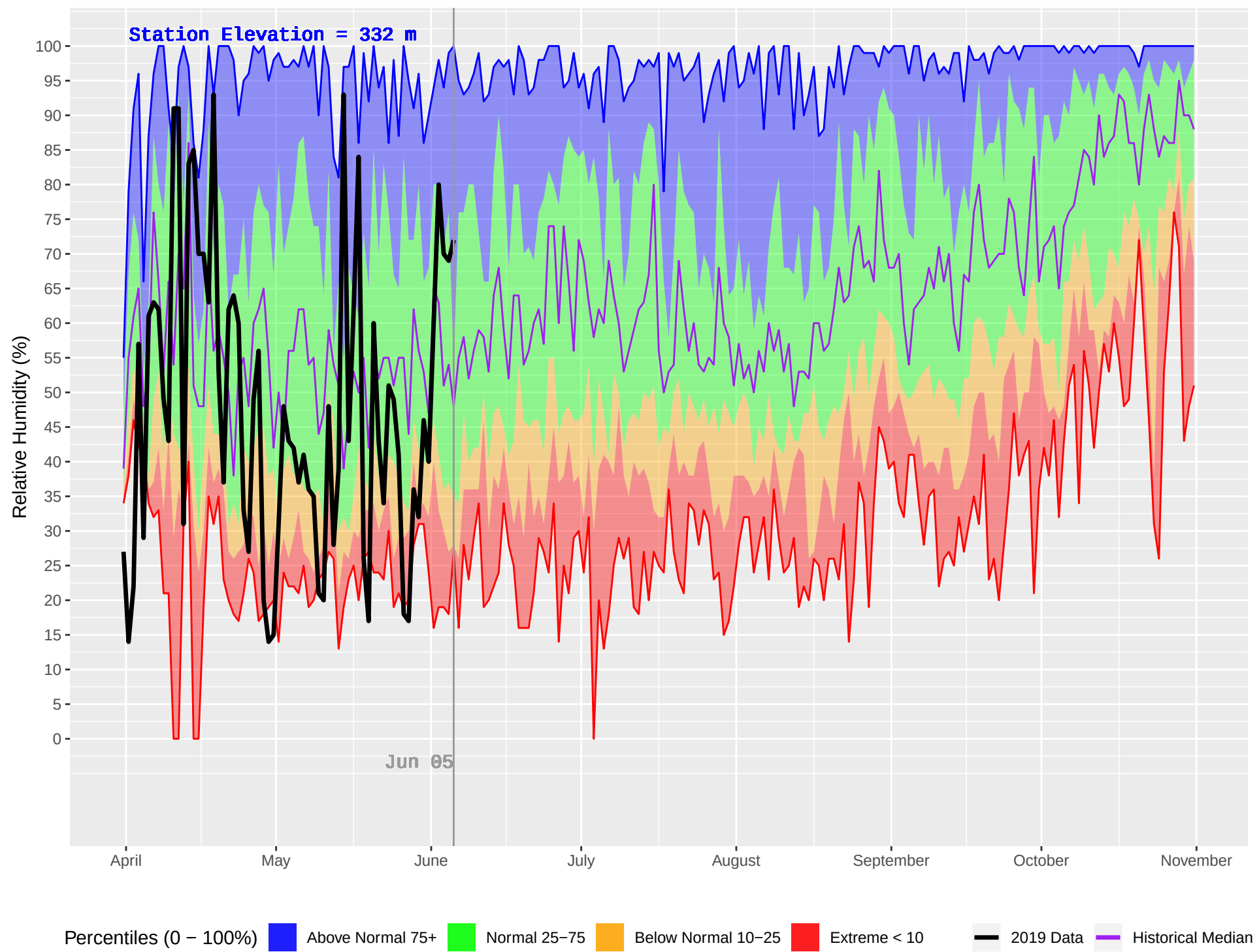
MACHMELL (101) : Historical (1990–2018) and Current (2019) Daily Relative Humidity
