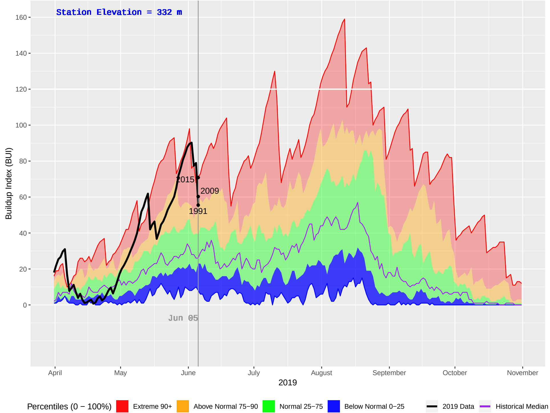
MACHMELL (101) : Historical (1990–2018), Current (2019) Daily Buildup Index (BUI)
