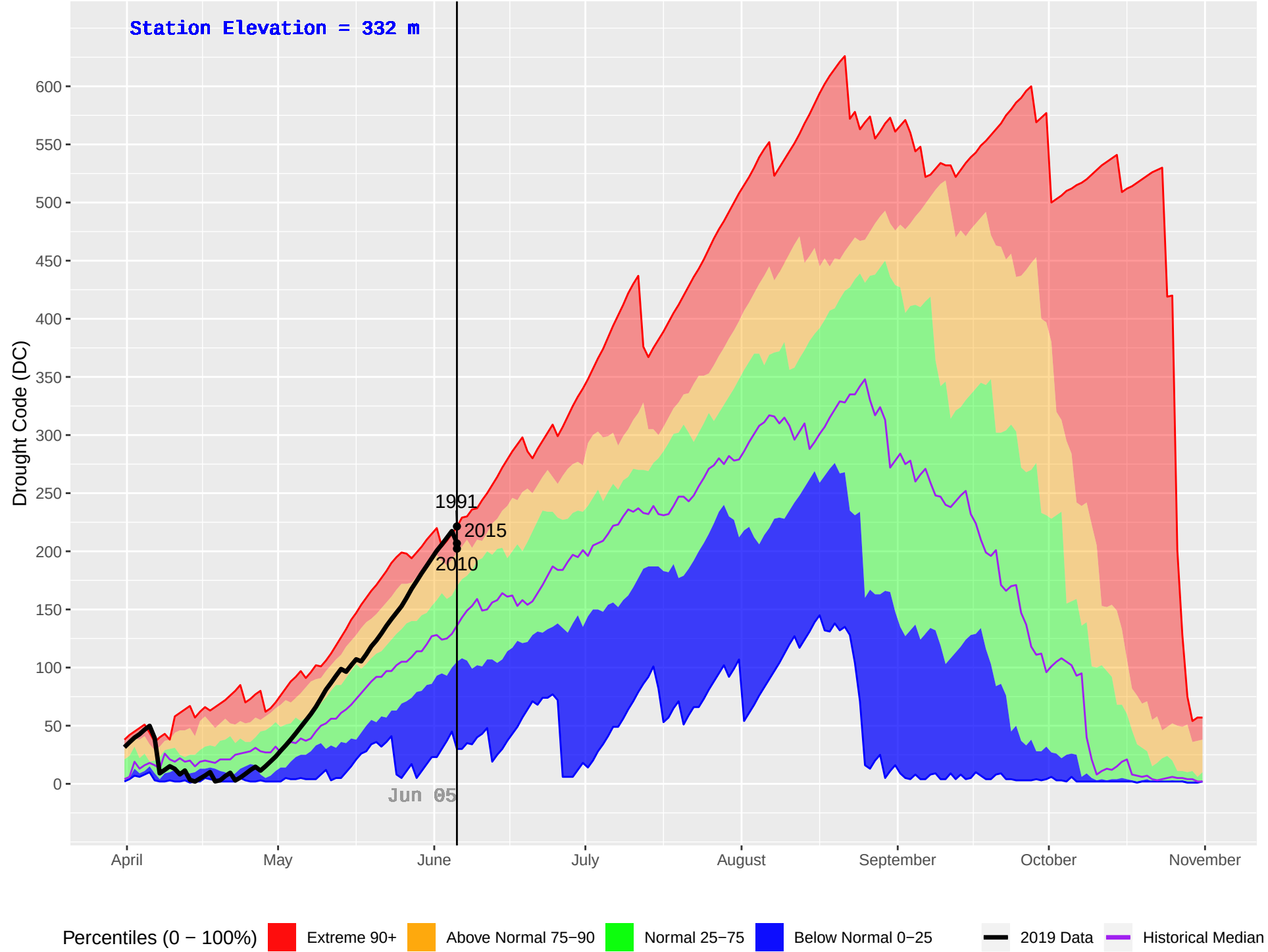
MACHMELL (101) : Historical (1990–2018) and Current (2019) Daily Drought Code (DC)
