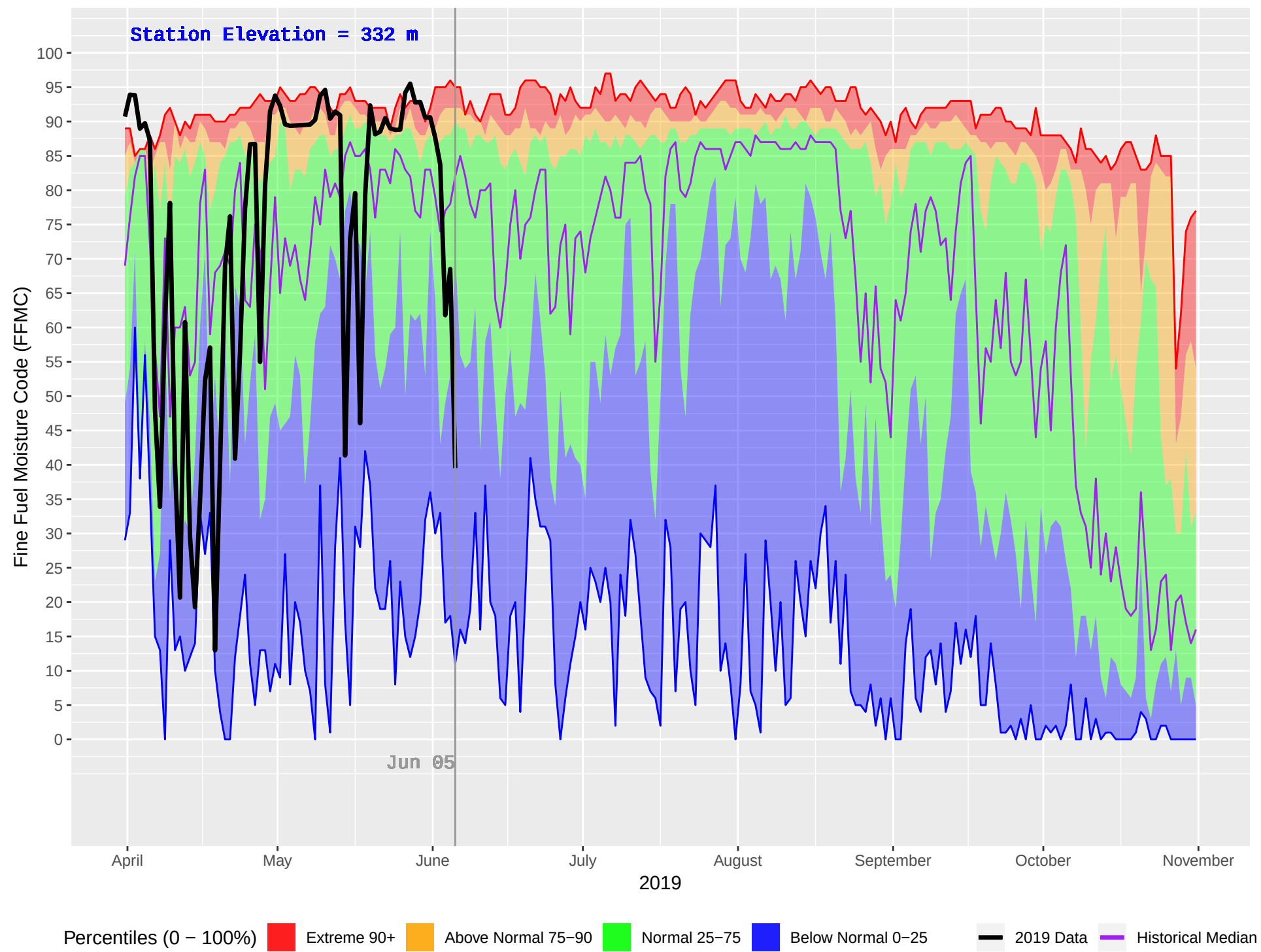
MACHMELL (101) : Historical (1990–2018) and Current (2019) Daily Fine Fuel Moisture Code (FFMC)
