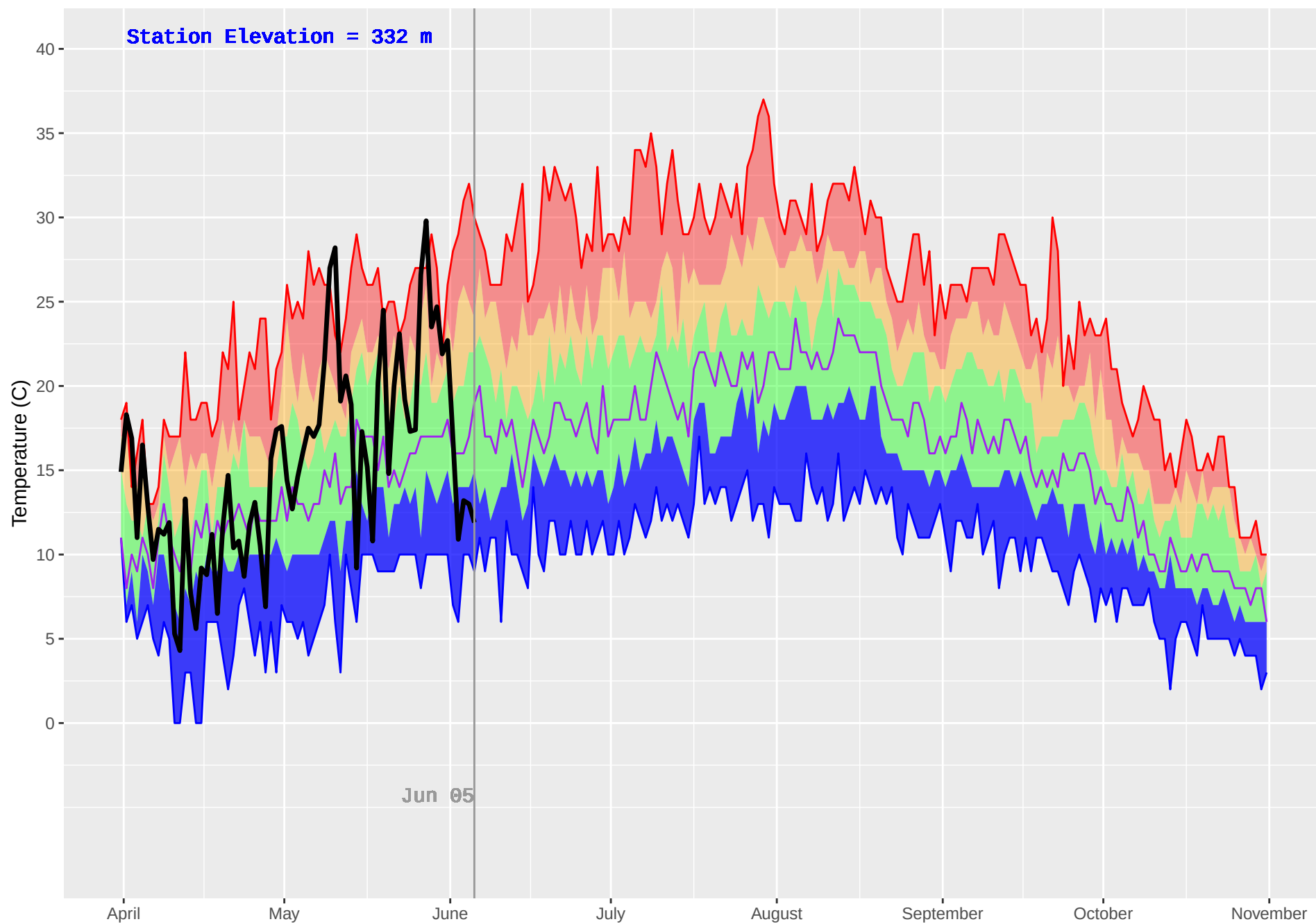
MACHMELL (101) : Historical (1990–2018) and Current (2019) Daily Temperature
