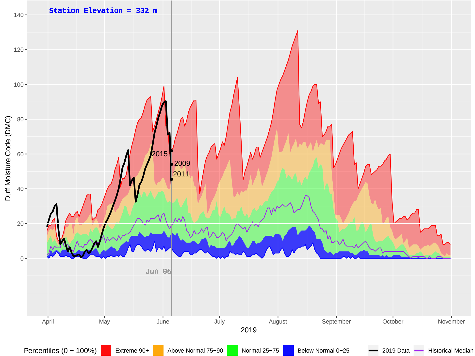
MACHMELL (101) : Historical (1990–2018), Current (2019) Daily Duff Moisture Code (DMC)
